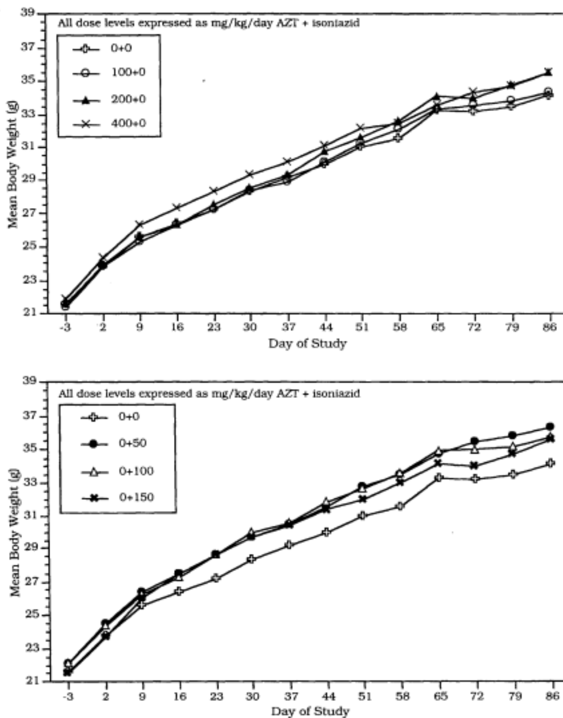
FIGURE 1 Mean Body Weights of Male (Core) Mice in the 13-Week Toxicity Study of AZT and Isoniazid Combinations
