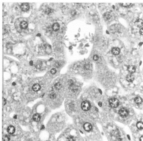
PLATE 6 Liver from a male mouse treated with 400 mg/kg AZT + 150 mg/kg isoniazid showing mild hepatocellular hypertrophy. ( \times 400 )
